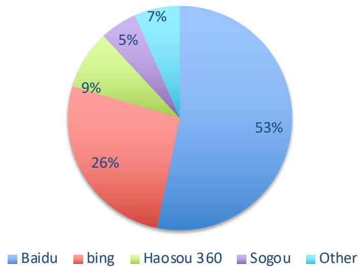
All Platforms
